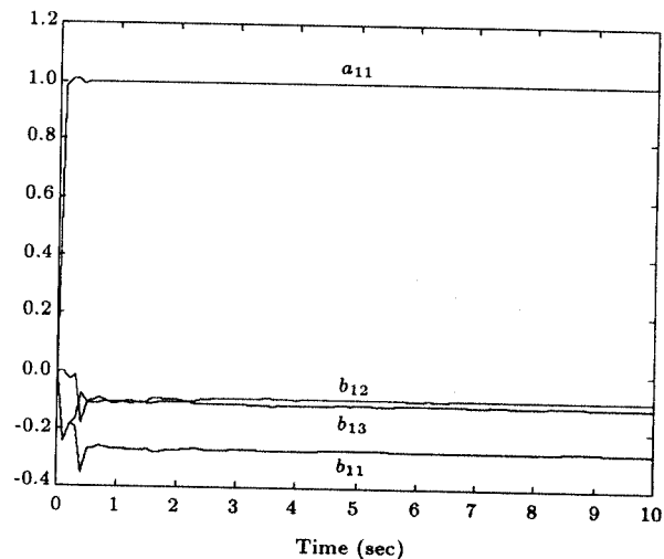
Figure 5. Off-line estimation of the unknown parameters of vector \hat{\theta}_1 (in 100 iterations or 10 fps).
