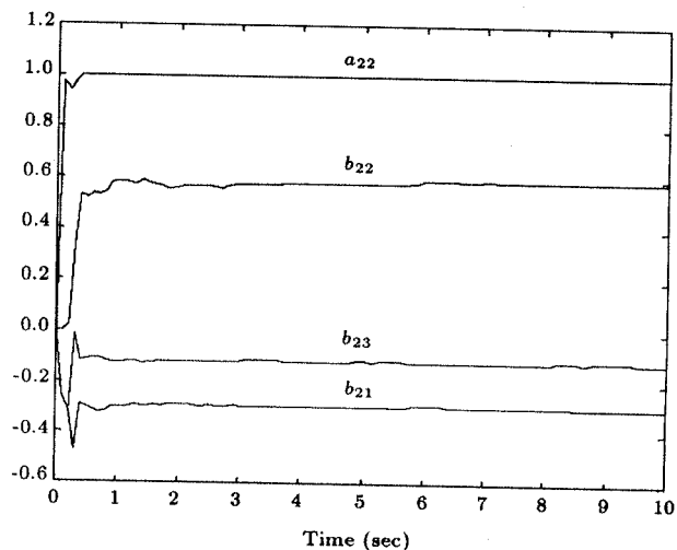
Figure 6. Off-line estimation of the unknown parameters of vector \hat{\theta}_2 (in 100 iterations or 10 fps).
