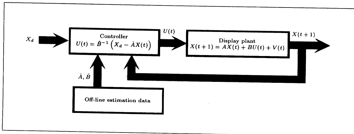
Figure 8. Block diagram of the auto-alignment system using off-line estimated model.
