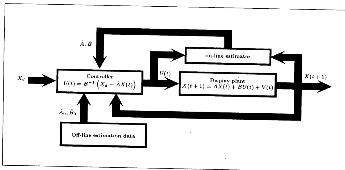
Figure 10. Block diagram of the authors' adaptive auto-alignment system using on-line estimator and off-line estimation data.
