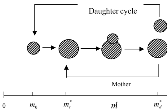
Fig. 1 Simplified cell cycle model for budding yeast
