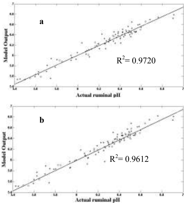
Fig 5. Correlation of neural network models output vs. actual ruminal pH values with training data set (69, *: training data) using the optimal network, with 1 hidden layer with 4 neurons and a test data set (23, o: test data). The y-axis represents the output of model vs. Actual pH on the x-axis. The scale from 5.4 to 7 on the y-axis and x-axis represent ruminal pH (a = time + C/F, and b = time +
