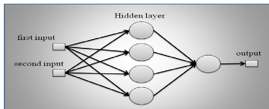
Fig 3. Selected neural network structure: two inputs were used for the artificial neural network (ANN): first input is time and the second input is concentrate to alfalfa hay ratios (60: 40, 70: 30, 80: 20 and 90: 10). For the ANN used to predict the ruminal pH, one output was used and the output value was the “ruminal pH”.
