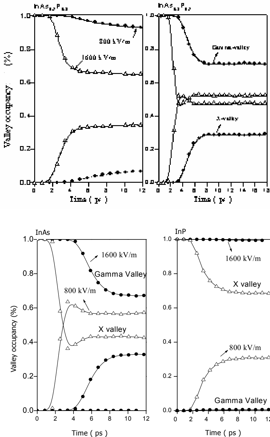
Figure 5. Comparison of the valley occupancy as a function of applied electric field in InAs, InP, \text{InAs}_{0.2}\text{P}_{0.8} and \text{InAs}_{0.8}\text{P}_{0.2} for \Gamma , X and L valleys at room temperature
