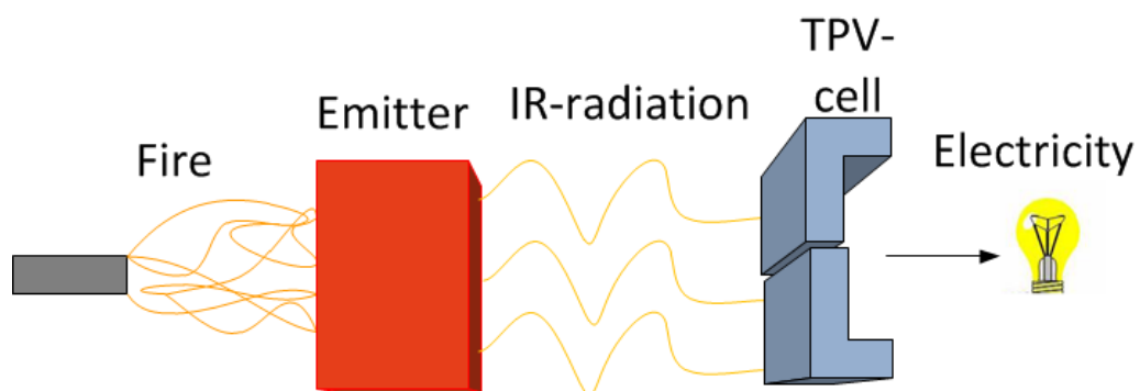
Fig. 1 Operating principle of a TPV device
