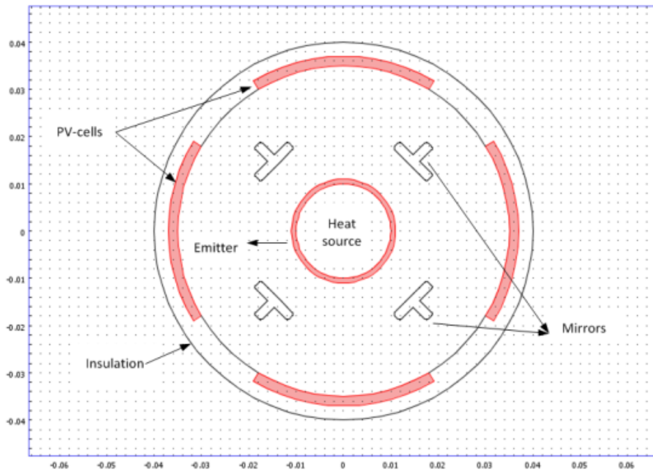
Fig. 2 Geometry and dimensions of the modeled TPV system
