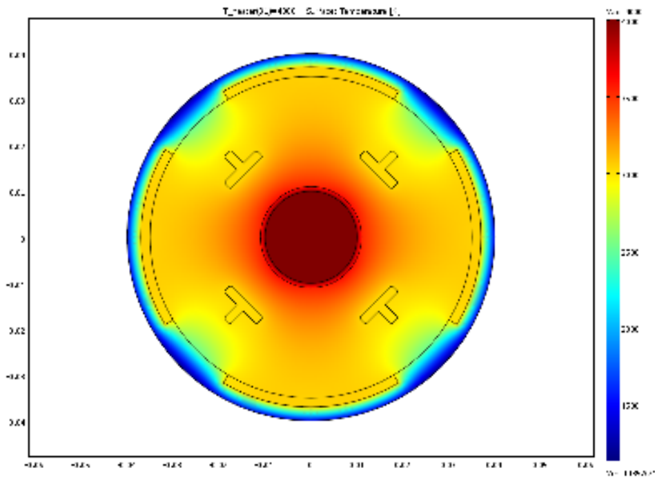
Fig. 3 Temperature distribution in the TPV system for 4000 °k as the emitter temperature.
