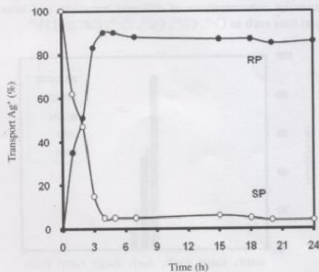
Fig. 7. Effect of time on silver transport. Experimental conditions: source phase, 10 mL of 5 \times 10^{-4} M \text{Ag}^+ at pH 6; liquid membrane phase, 50 mL of 2 \times 10^{-3} M \text{C}_{20}\text{H}_{38}\text{O}_4\text{S}_2 carrier and 4 \times 10^{-3} M of palmitic acid in 1,2-dichloroethane; receiving phase, 20 mL of 0.01 M \text{S}_2\text{O}_3^{2-} at pH 5
