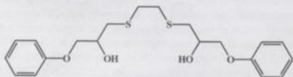
Scheme-I: Structure of 2,9-dihydroxy-1,10-diphenoxy-4,7-dithia decane (C 20 H 26 O 4 S 2 )
