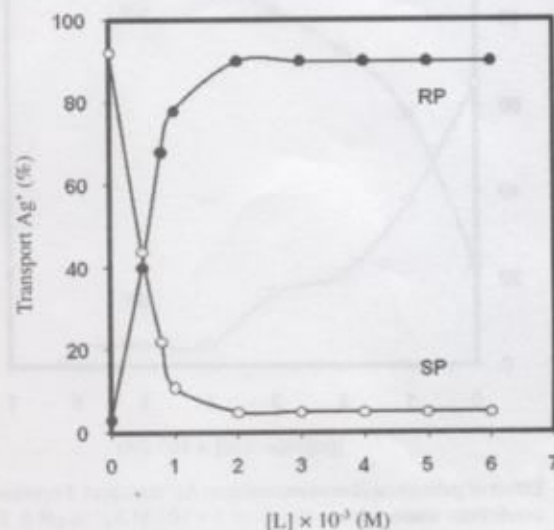
Fig. 1. Effect of carrier concentration on silver(I) cation transport. Experimental conditions: source phase, 10 mL of 5 \times 10^{-4} M Ag^+ at pH 6; liquid membrane phase, 50 mL of varying concentration of C_{20}H_{36}O_4S_2 carrier and 4 \times 10^{-3} M palmitic acid in 1,2-dichloroethane; receiving phase, 20 mL of 0.01 M S_2O_3^{2-} at pH 5; time of transport, 4 h
