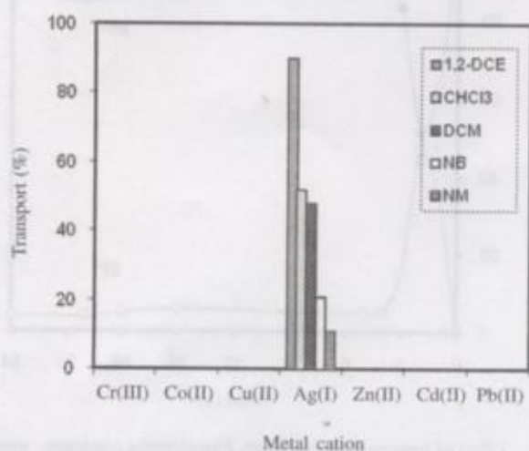
Fig. 8. The results of metal ion transport. Experimental conditions: source phase, 10 mL of 5 \times 10^{-4} M of metal cations at pH 6; liquid membrane phase, 50 mL of 2 \times 10^{-3} M C_{20}H_{38}O_4S_2 carrier and 4 \times 10^{-3} M of palmitic acid in different organic solvent; receiving phase, 20 mL of 0.01 M S_2O_3^{2-} at pH 5; time of transport, 4 h
