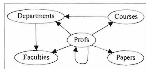
Figure 2. Interlinking of FUM-LD dataset
