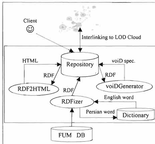
Figure 1. FUM-LD Framework
