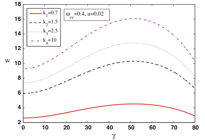
Fig. 3 Soliton width as functions of l_z with different values for the parameter “ \kappa ”
