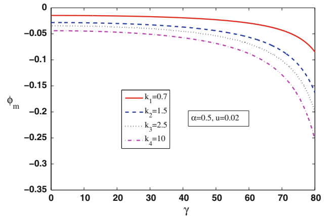
Fig. 1 Soliton amplitude \phi_m respect to \gamma with different values for the parameter “ \kappa ”
