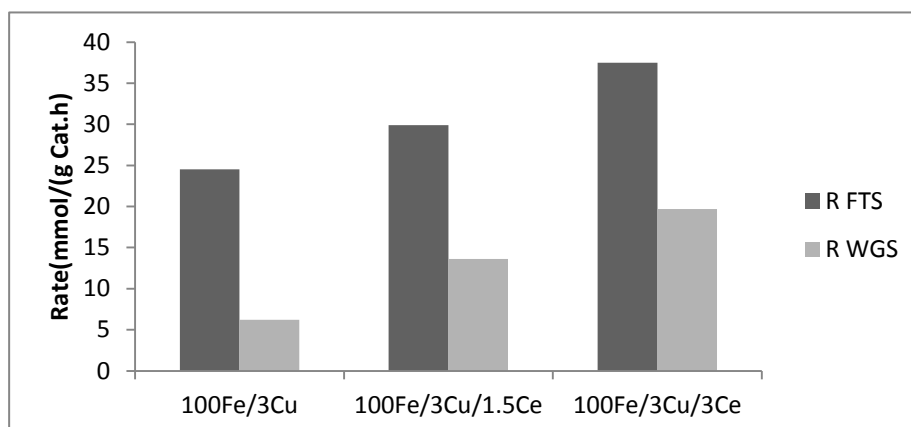
Figure 5: R_{FTS} and R_{WGS} of the catalysts
