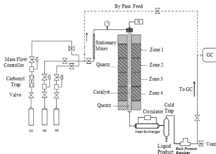
Figure 1: Cata - test system
