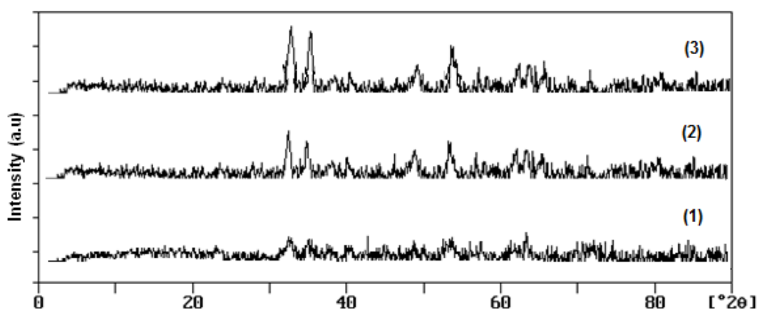
Figure 2: XRD spectra of the fresh catalysts: (1) 100Fe/3Cu (2) 100Fe/3Cu/1.5Ce (3) 100Fe/3Cu/3Ce
