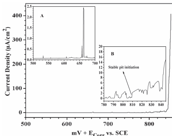
Fig. 4. Slow ramp anodic polarization of electropolished 316 StSt with 3mV/min scanning rate in potential range of 500-860 mV higher than E_{corr} (inserted micrograph A shows results in a range of 500-700 mV higher than E_{corr} and B shows potential which is stable pit initiated on surface)
