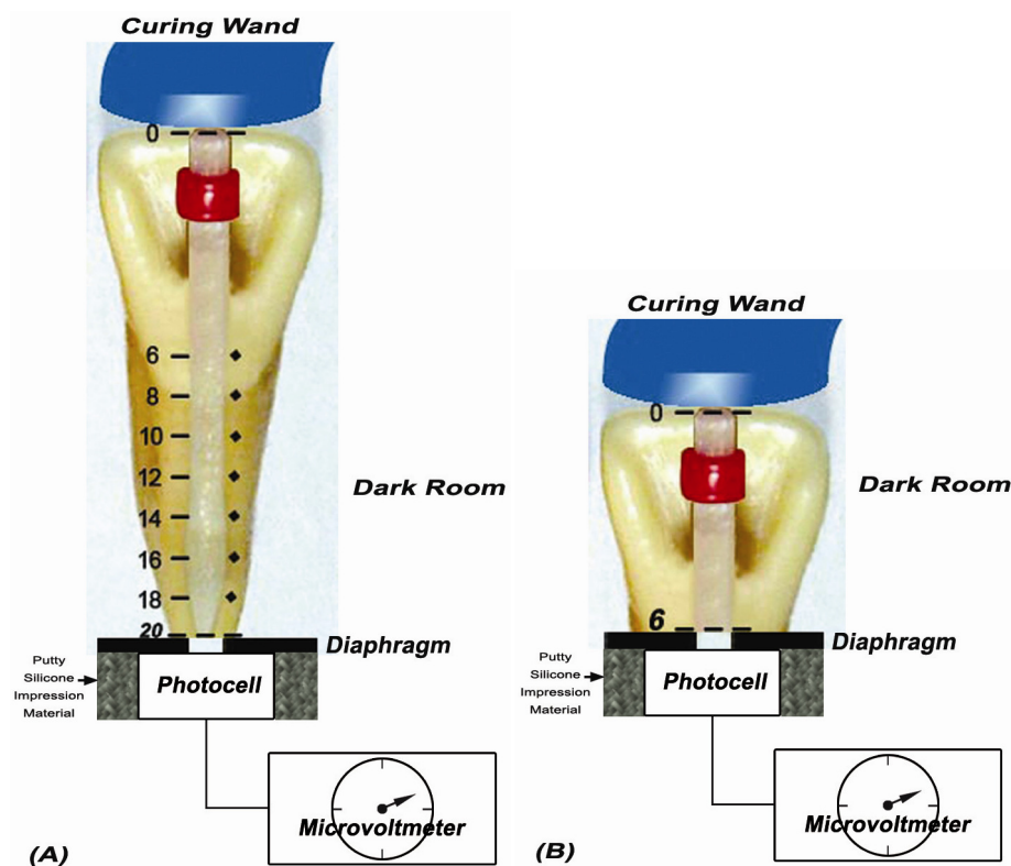
Figure 1. Schematic illustration of light intensity measurement at different depths (A: 16 mm, B: 6 mm)
