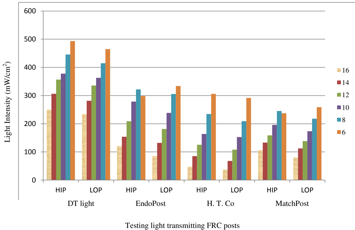
Figure 2. Light intensity ( \text{mW}/\text{cm}^2 ) in different thicknesses of testing light transmitting FRC posts
