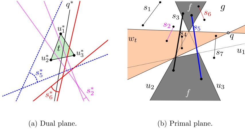
Figure 4: (a) In the dual plane, the triangle t , is intersected by q^* . The dual of some of obstacle segments are also shown. (b) The arrangement of f , g , q and segments of S in the primal plane.
