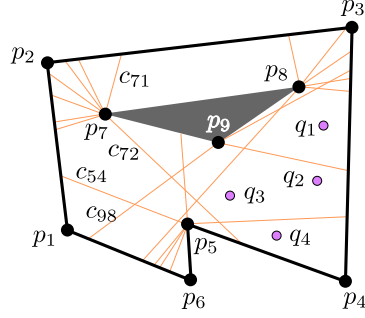
Figure 1: Visibility decomposition for a polygonal domain. q_1 , q_2 and q_4 have different combinatorial visibilities, while q_2 and q_3 have similar combinatorial visibilities.
