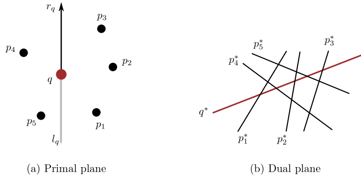
Figure 3: (a) A set of points P = \{p_1, p_2, p_3, p_4, p_5\} and a point q in the primal plane. (b) The dual lines of points of P and q .
