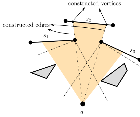
Figure 2: Parts of the VP of a point. Colored region denotes VP(q) . The constructed edges and constructed vertices of the VP are marked.
