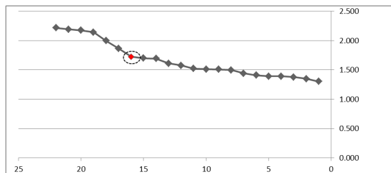
Figure 3. Line graph for coefficients of the final 22 steps of the single linkage clustering.
