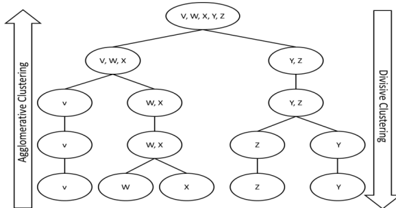
Figure 1. Agglomerative and divisive clustering.
