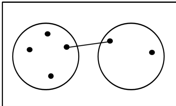
Figure 2. The single linkage procedure for calculating distance between clusters. PRACTICE in CLINICAL PSYCHOLOGY
