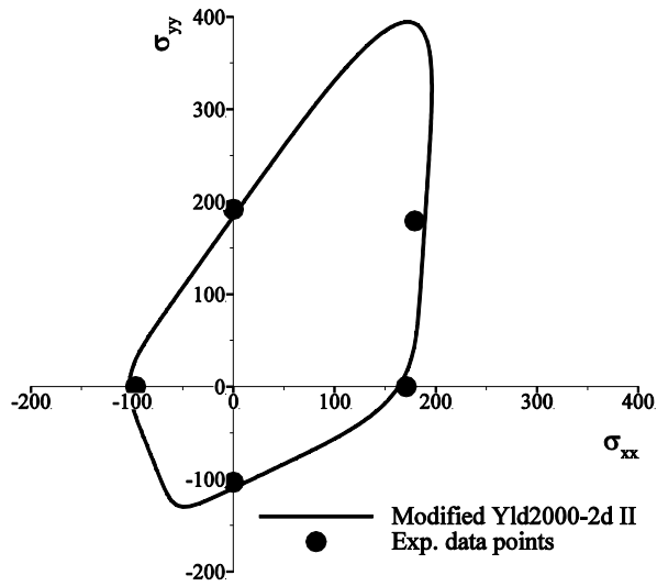
Figure 7: The Modified Yld2000-2d II and experimental data points for AZ31.
