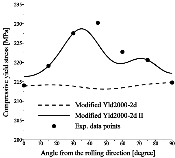
Figure 3: Comparison of the yield stress directionality for Al 2008-T4: (a) uniaxial tensile yield stress; and (b) uniaxial compressive yield stress.
