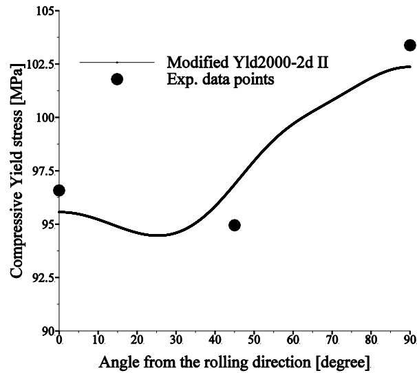
Figure 8: Comparison of the Modified Yld2000-2d II with experimental results for AZ31: (a) uniaxial tensile yield stress, (b) uniaxial compressive yield stress.
