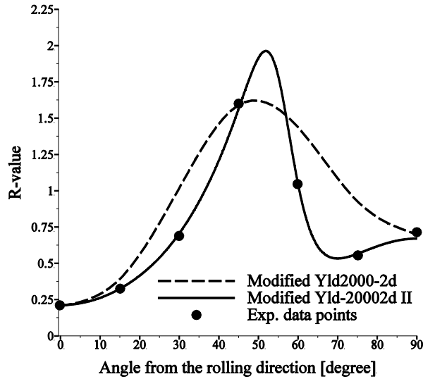
Figure 6: Comparison of the R -value directionality for Al 2090-T3.
