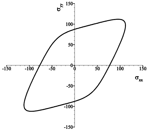
Figure 1: (a) Yield function of Modified Yld 2000-2d and Modified Yld 2000-2d II in compared with experimental results, (b) plastic potential surface of Modified Yld 2000-2d II for Al 2008-T4.
