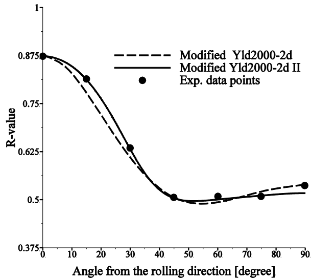
Figure 5: Comparison of the R -value directionality for Al 2008-T4.
