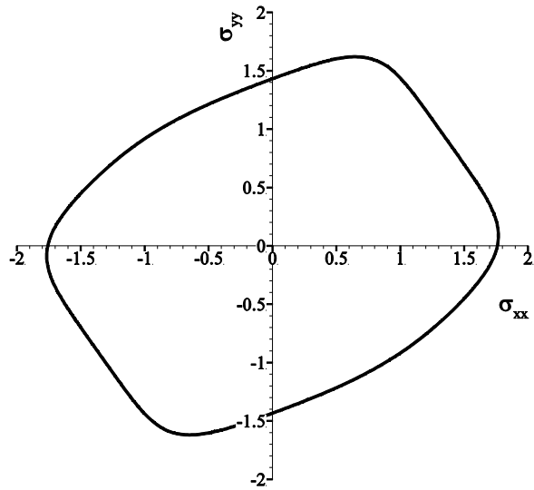
Figure 2: (a) Yield function of Modified Yld 2000-2d and Modified Yld 2000-2d II in compared with experimental results, (b) plastic potential surfaces of Modified Yld 2000-2d II for Al 2090-T3.
