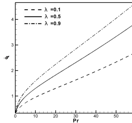
Fig. 18. Dimensionless temperature gradient distributions at \eta = 0.0 versus Pr number in terms of selected values of \lambda parameter when S = 0.1 .
