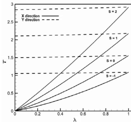
Fig. 13. Distributions of shear stress components in x and y directions in terms of different values of \lambda and S parameters when \gamma = 0.0 .
