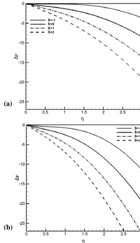
Fig. 6. Distributions of pressure profiles for different values of S parameter when (a) \lambda = 0.1 and (b) \lambda = 0.9 .
