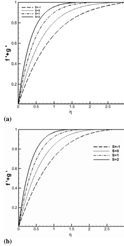
Fig. 3. Distributions of f'+g' profiles for different values of S parameter when (a) \lambda = 0.1 and (b) \lambda = 0.9 .
