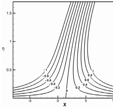
Fig. 12. Streamlines in x-\eta plane for the case of \gamma = -2.0 when \lambda = 0.5, S = 0.0 .
