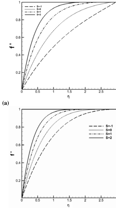
Fig. 2. Distributions of f' profiles for different values of S parameter when (a) \lambda = 0.1 and (b) \lambda = 0.9 .
