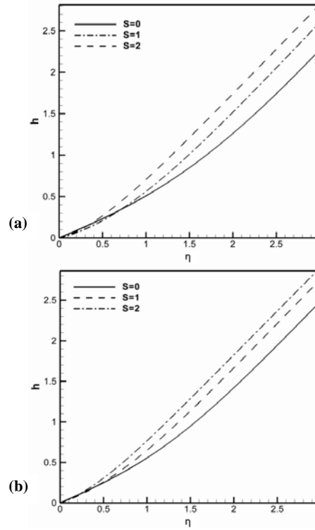
Fig. 5. Distributions of h(\eta) profiles for different values of S parameter when (a) \lambda = 0.1 and (b) \lambda = 0.9 .
