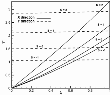
Fig. 14. Distributions of shear stress components in x and y directions in terms of different values of \lambda and S parameters when \gamma = 1.0 .
