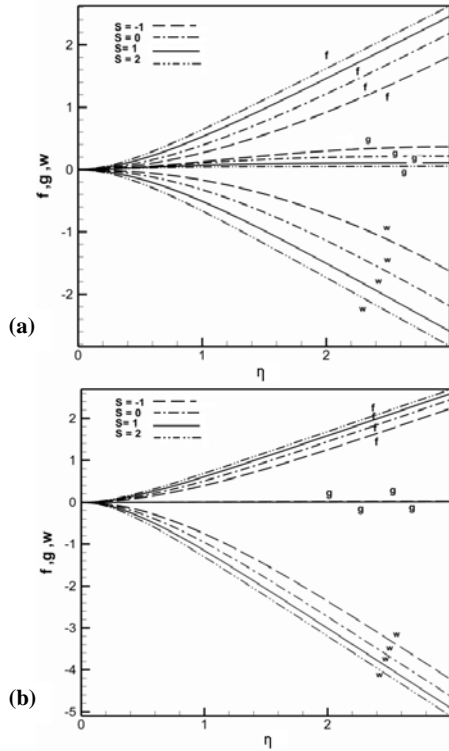
Fig. 4. Distributions of w-component of velocity, f(\eta) and g(\eta) functions for different values of S parameter when (a) \lambda = 0.1 and (b) \lambda = 0.9 .
