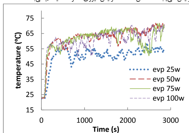
Fig. 4 Evaporator temperature vs. time for heat input
