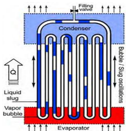
Fig. 1 Schematic of pulsating heat pipe
