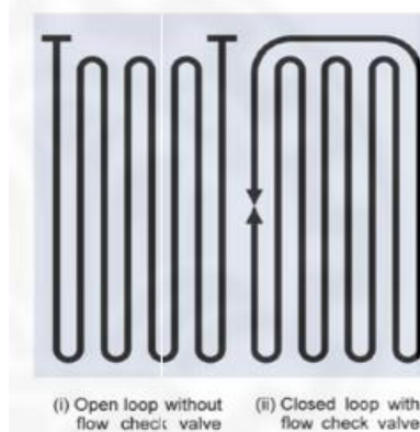
Fig. 2 Schematic of open and closed loop pulsating heat pipe
