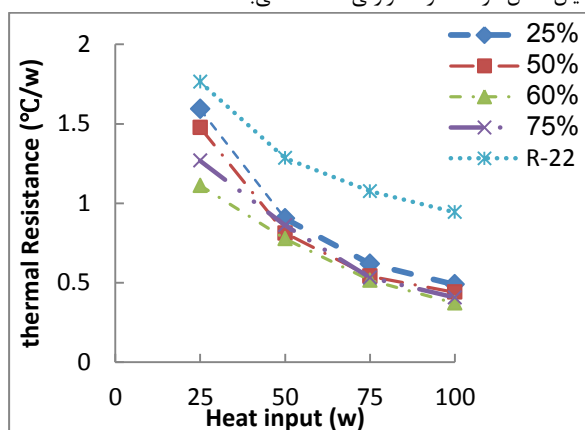
Fig. 5 Variation of thermal resistance with heat power
