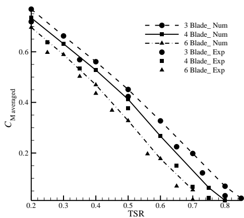
Fig.15 Numerical averaged torque coefficients, C_{Maveraged} , as a function of TSR, in comparison with the experimental data for the rotors with different number of blades
