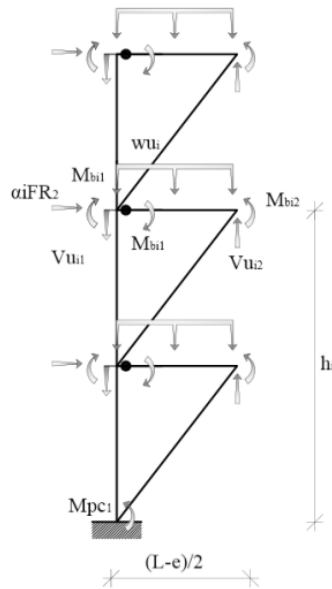
Figure 5: Lateral force for designing of out of link member in braced frame.
