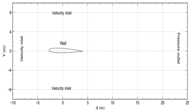
Fig. 1. Computational region and boundary conditions for airfoil
