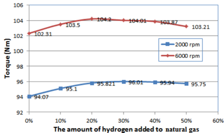
Fig. 11. Torque versus the amount of hydrogen added to natural gas and spark timing of 19°C BTDC at 2000 rpm and spark timing of 28°C BTDC at 6000 rpm
