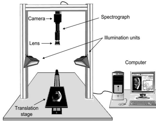
Fig. 1. Configuration of the hyperspectral imaging system.
