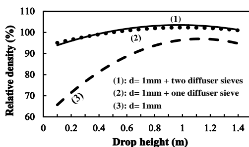
Figure 13. Effect of drop height on relative density (Third part of the Section II)
