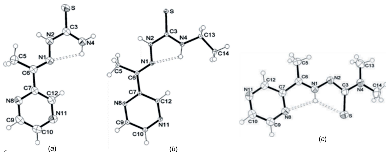
Figure 6 Displacement ellipsoid plots (50% probability) of three thiosemicarbazones. Reproduced from Venkatraman et al. (2009) with permission.
