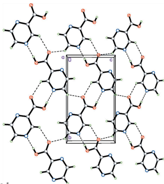
Figure 1 The 1D zigzag chains and 2D structure of pyrazine-2-carboxylic acid formed by O—H...N and C—H...O hydrogen bonds (dashed lines) between adjacent molecules. Reproduced from Shi et al. (2006) with permission.
