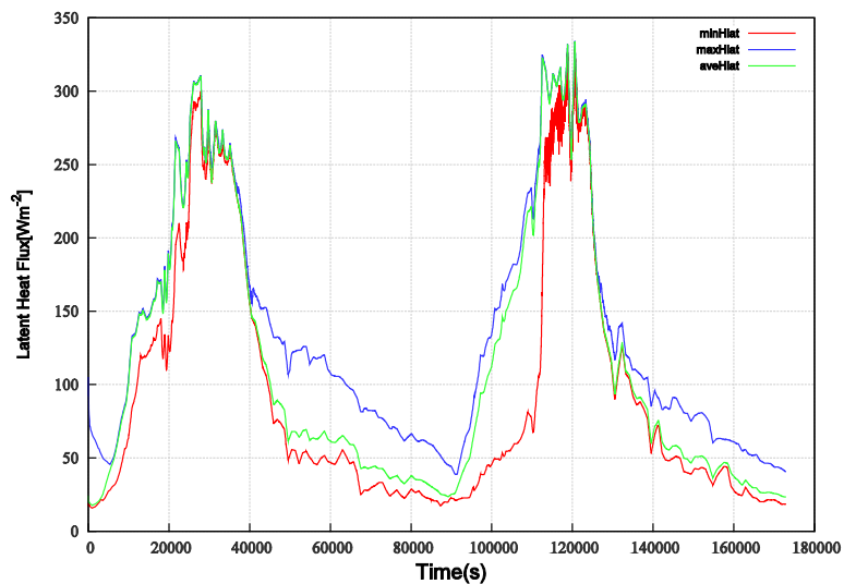
Figure 3. Maximum, minimum and average values of calculated latent heat flux over the water surface
