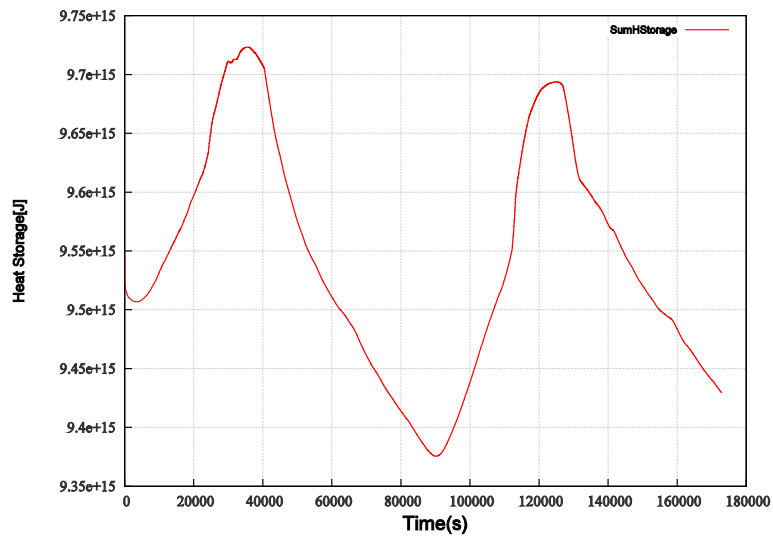
Figure 4. Calculated heat storage of lake to use in evaporation estimation from water surface
