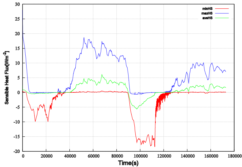
Figure 2. Maximum, minimum and average values of sensible heat flux over the water surface
