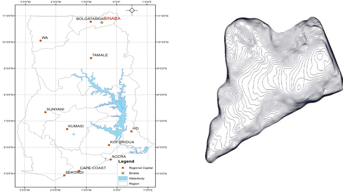
Figure 1. a) Location of Lake Binaba in the Upper East region of Ghana. b) Bathymetry map of the lake with depth contours.
