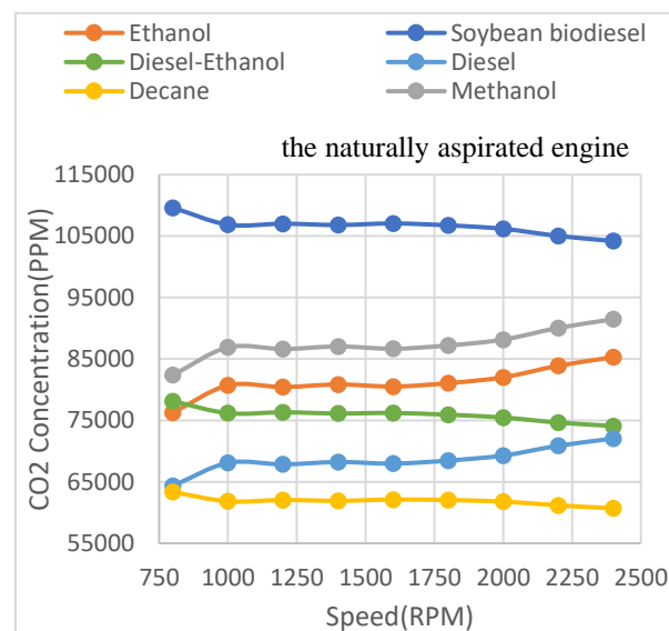
Fig.7. CO 2 emission in turbocharged and the naturally aspirated engine with different fuels
