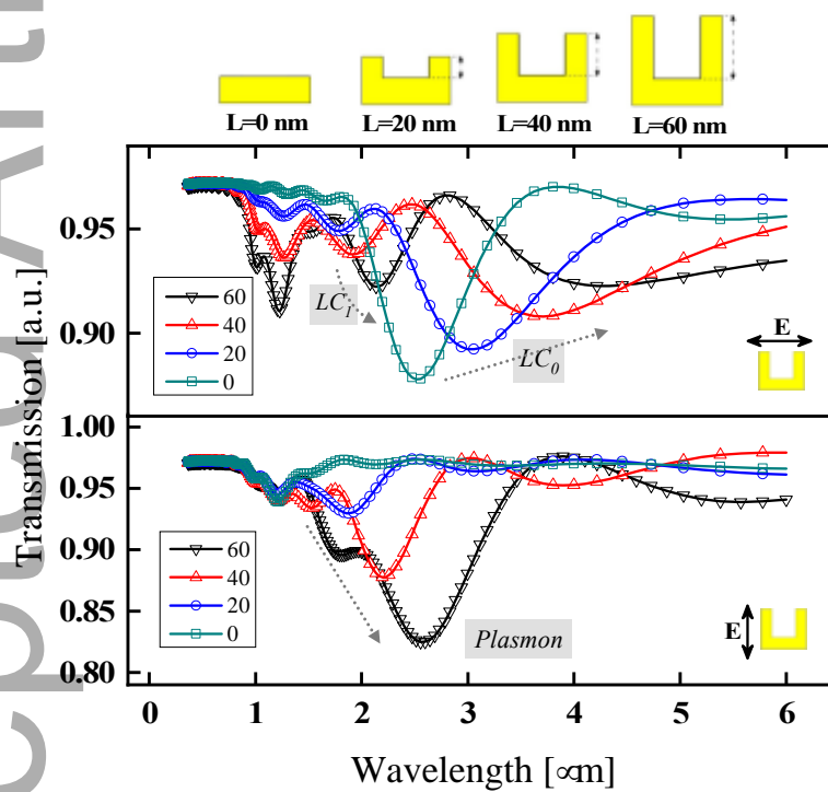
Figure 8. The calculated optical transmission spectra of AZOU6 SRRs with respect to different lengths of the vertical arm (top panel) for 85 nm-sized resonators.
