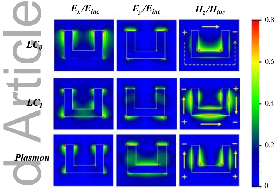
Figure 9. Calculated relative electric and magnetic field amplitudes, for 85 nm-size AZOU6 SRRs, where E_{inc} and H_{inc} denote the incident electric and magnetic field amplitudes, respectively. The yellow arrows indicate electric dipole moments. The LC modes are associated with the polarization along the horizontal arm while Plasmon mode was excited in the polarization parallel to the side arms.
