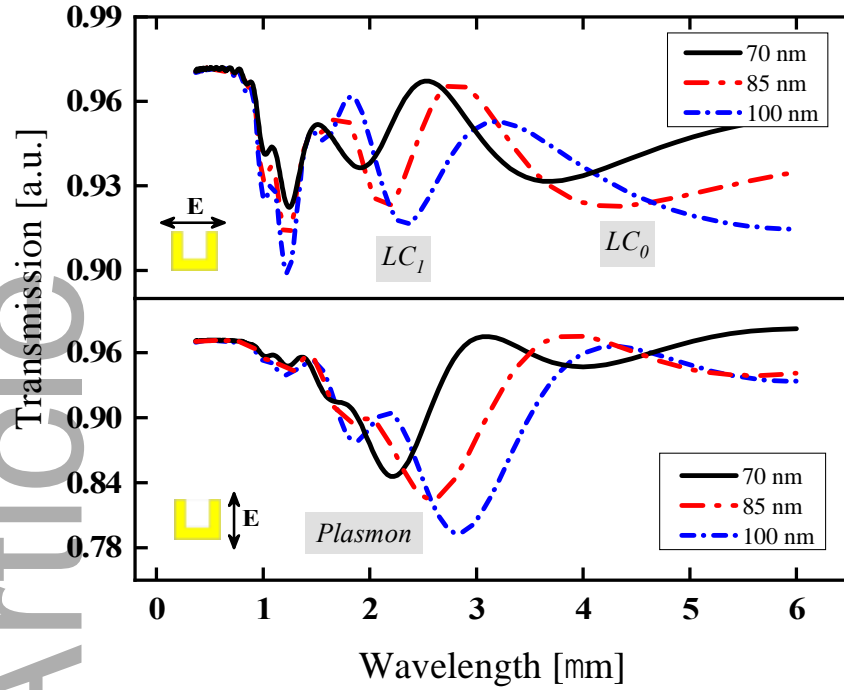
Figure 7. Optical transmission spectra calculated for the proposed AZOU6 SRRs with respect to differently sized resonators.
