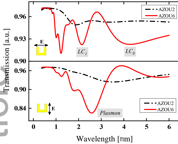
Figure 6. The calculated optical transmission spectra of 85 nm sized u-shaped SRRs for the proposed AZOU2 and AZOU6 compounds as the constituting material. Plasmon and LC modes are clearly excited in the system.
