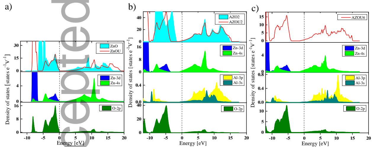
Figure 2. The calculated DOS and PDOS of ZnO (a), AZO2 (b) and AZO6 (c) with and without Hubbard model ( U ). The PDOS curves were only depicted for the compounds with Hubbard correction included. The Fermi level was set at zero energy.
