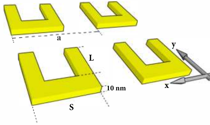
Figure 5. A schematic of a cell containing a square array of four u-shaped AZO SRRs. The periodic lattice constant and size of resonators are shown by a and S , respectively.
