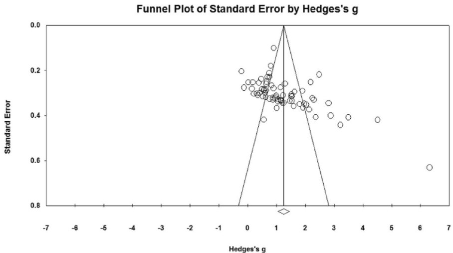
Fig. 1 Funnel plot under random-effects model
