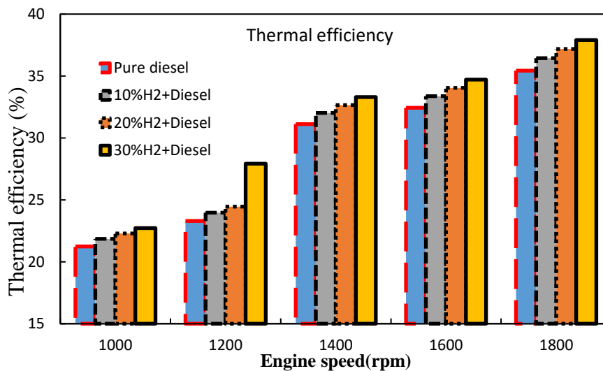
Fig 5. Variations of thermal efficiency versus engine speed with adding hydrogen to diesel fuel
