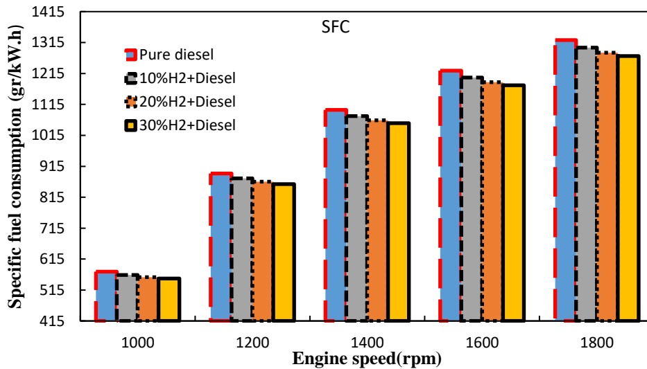
Fig 8. Variation of engine specific fuel consumption versus engine speed by adding hydrogen to diesel fuel
