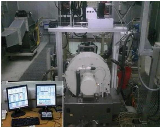
Fig 3. Control panel and test engine on dynamometer
