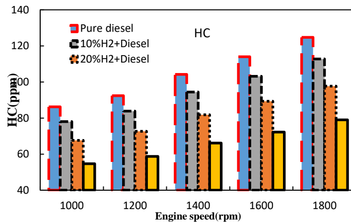
Fig 11. Variation of HC emissions versus engine speed with adding hydrogen to diesel fuel
