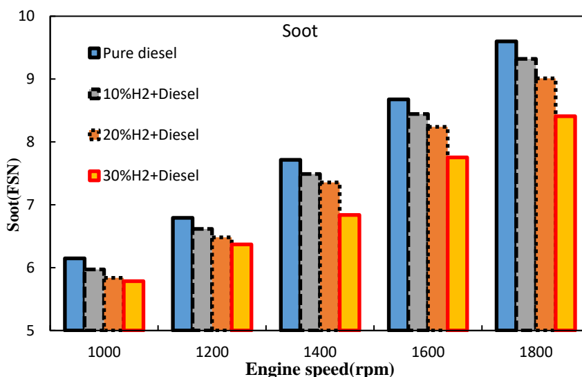
Fig 10. Variation of soot emissions versus engine speed with adding hydrogen to diesel fuel
