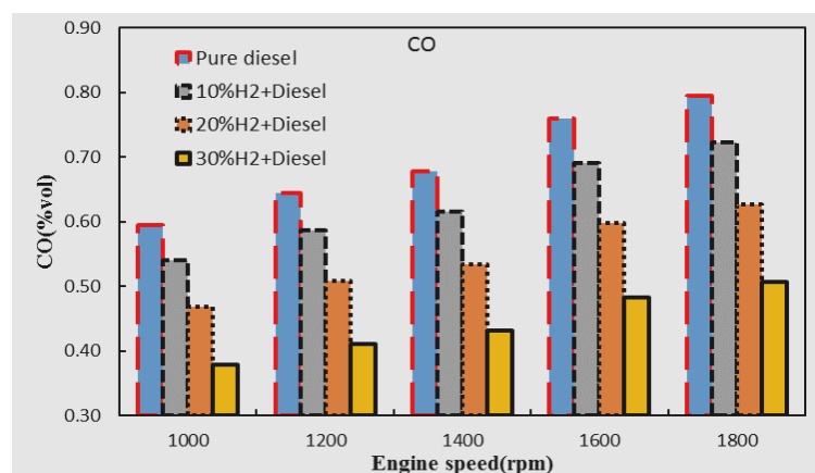
Fig 12. Variation of CO emissions versus engine speed with adding hydrogen to diesel fuel
