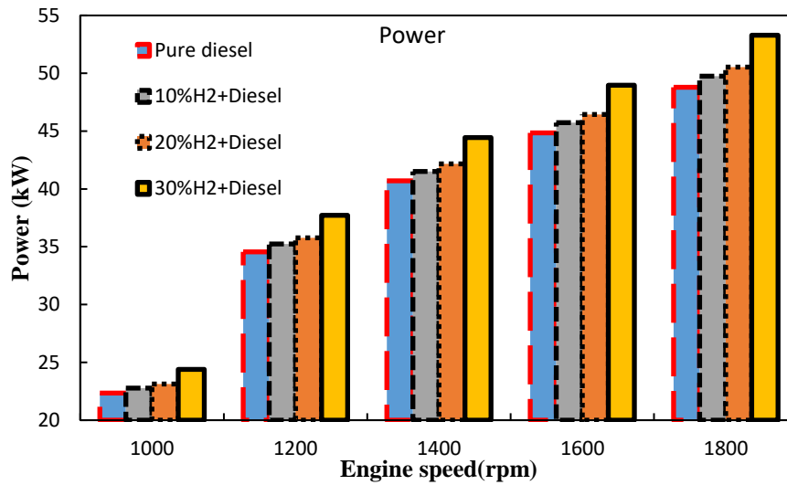
Fig 7. Variation of engine power versus engine speed with adding hydrogen to diesel fuel
