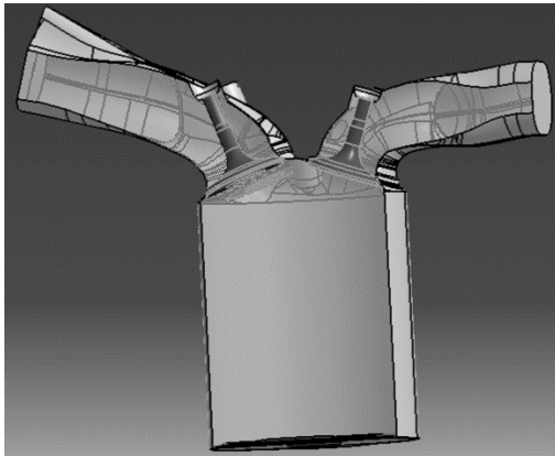
Fig 1. The geometry of the model designed for a diesel engine.
