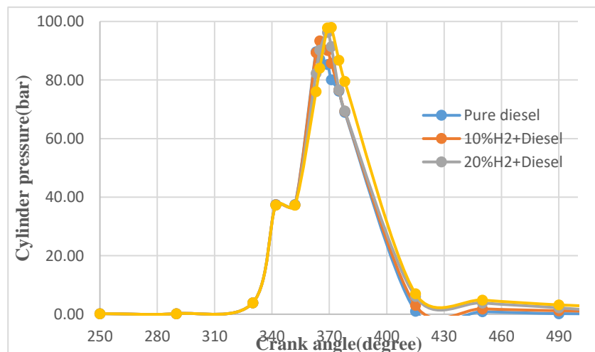
Fig 6. Variation of cylinder pressure versus crank angle with adding hydrogen to diesel fuel
