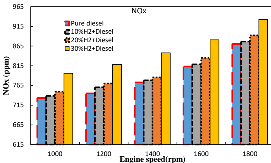
Fig 9. Variation of NOx emissions versus engine speed with adding hydrogen to diesel fuel
