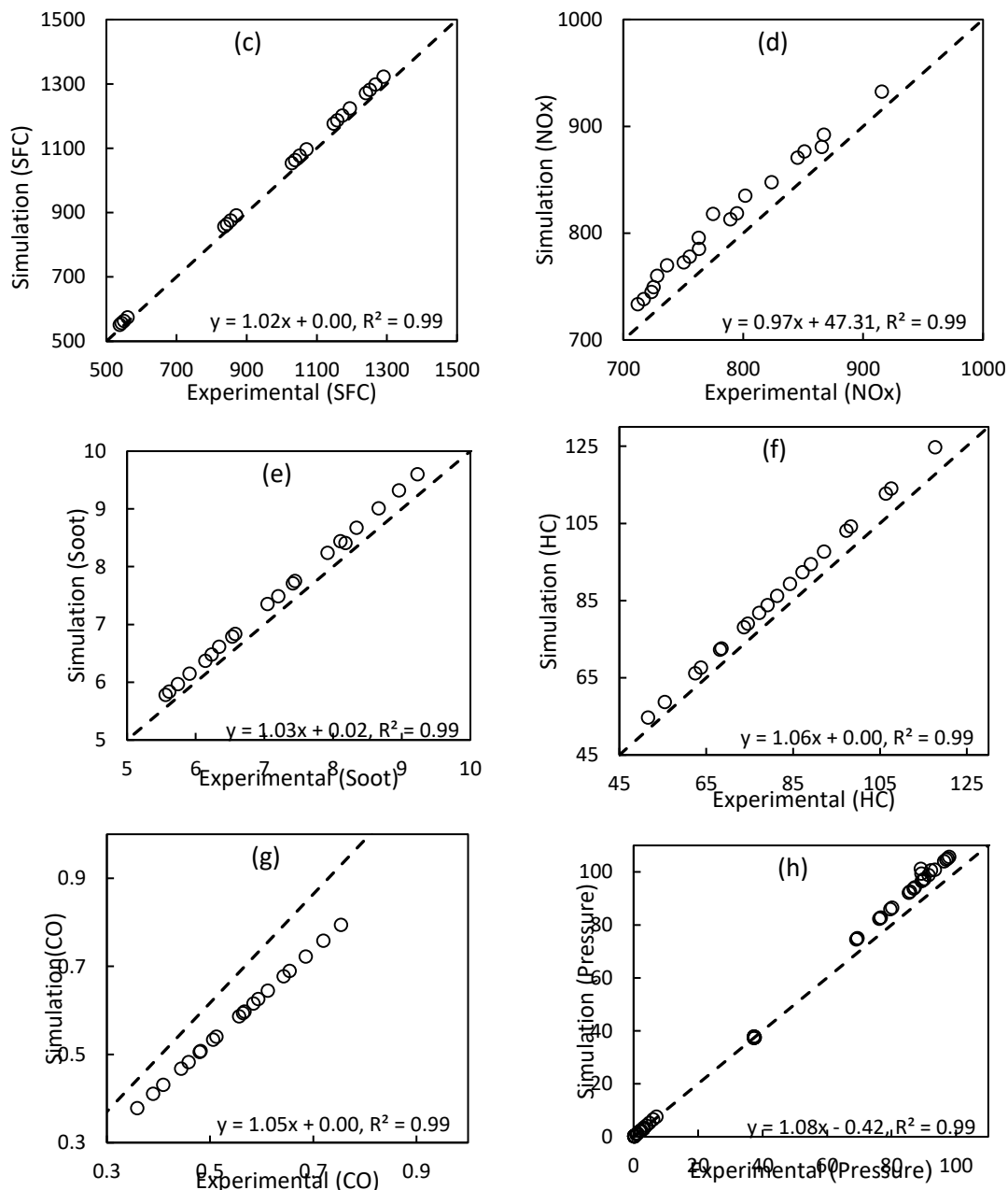
Fig.4 comparison between simulation and experimental data
