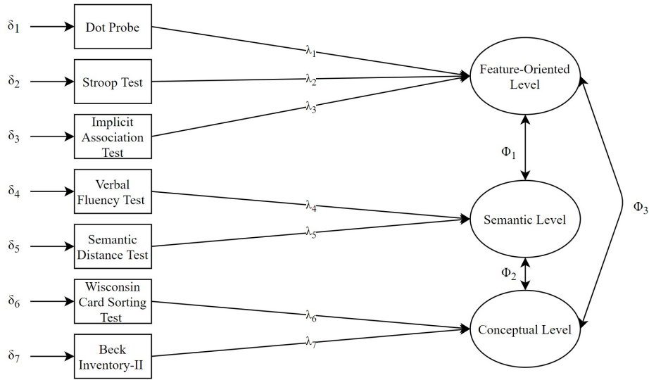
Figure 3. SEM specification for the proposed integrative model.
