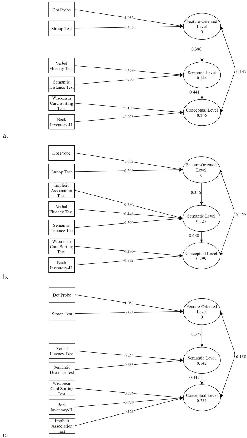
Figure 4. SEM specification for the proposed model.
