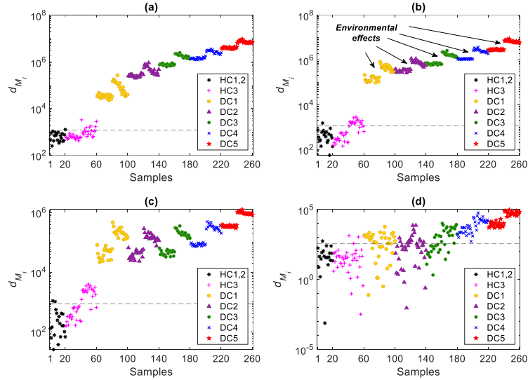
Fig. 3. Damage detection by the multi-stage ML methodology and the AR spectrum, avoiding to exploit the capability of the AANN to remove the environmental variability: (a) scenario 1, (b) scenario 2, (c) scenario 3, (d) scenario 4
