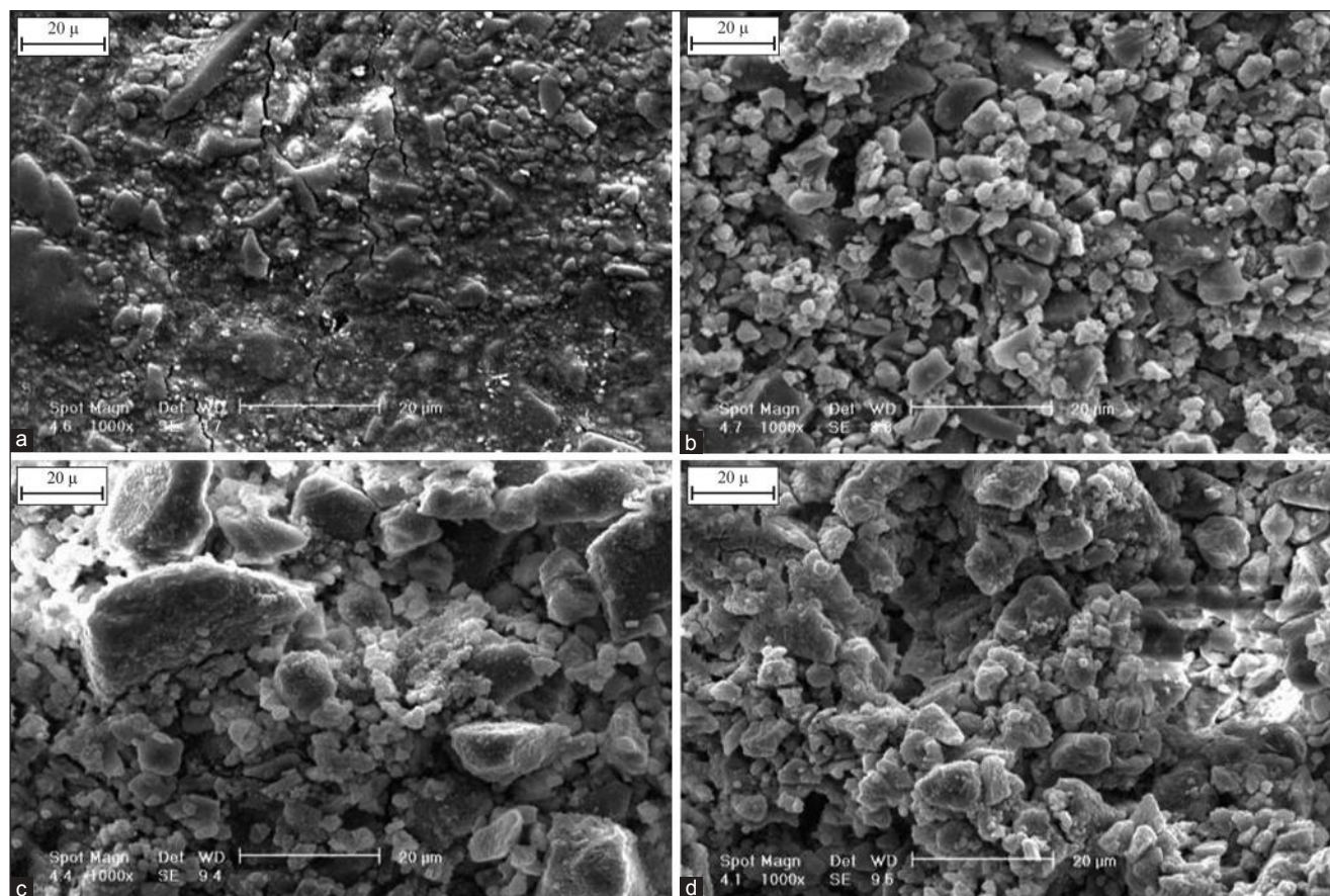
Figure 7: Scanning electron microscopy photograph of the glass ionomer cement (GIC) containing 3wt.% \text{Mg}_2\text{SiO}_4 nanoparticles before (a) and after 7 days (b), 14 days (c) and 21 days (d) immersion in simulated body fluid solution (1000 \times )
