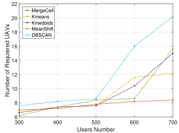
(a) Number of required UAVs.
