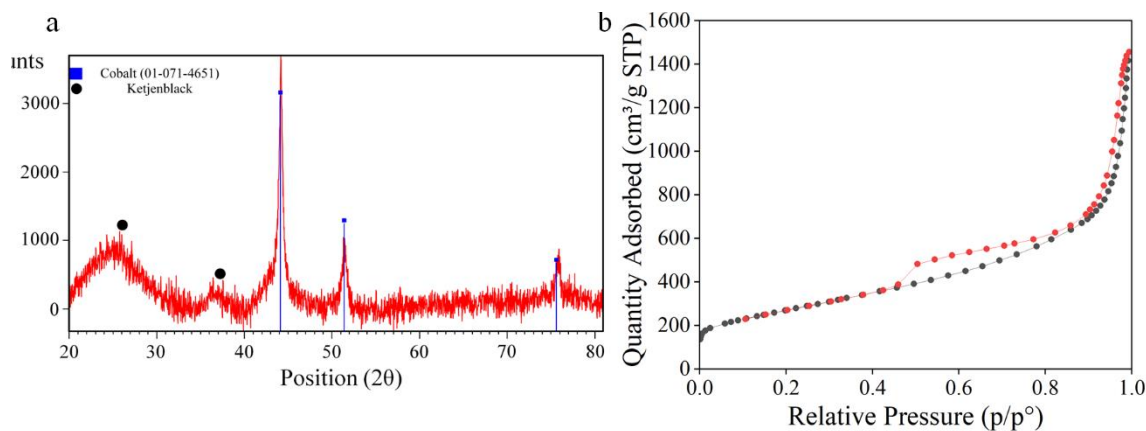
Fig. 2- (a) XRD patterns of Co@KB composite (b) \text{N}_2 adsorption.
