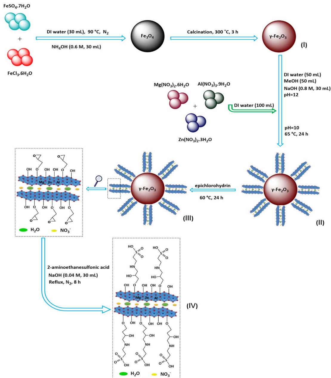
Scheme 1 Preparation steps of \gamma -Fe 2 O 3 @Zn-LDH-EAE-SO 3 H (IV).
