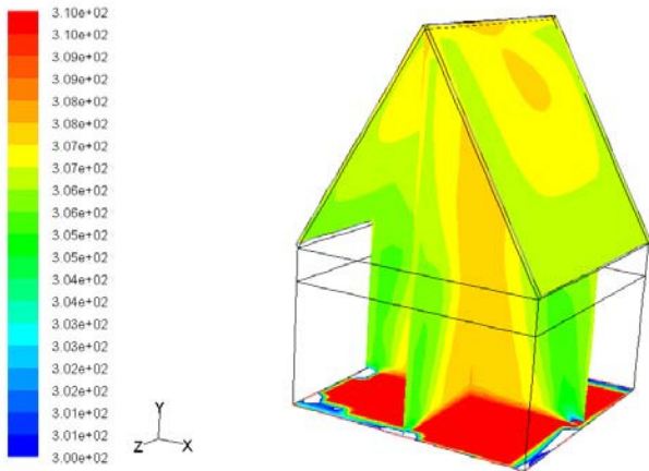
Figure.4 temperature distribution(k) Injecting from whole surface with flow rate 1.27 kg/s
