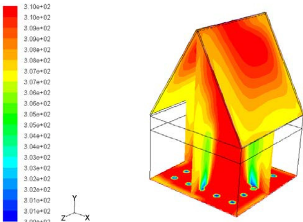
Fig.8 temperature distribution(k) with flow rate 0.85 kg/s
