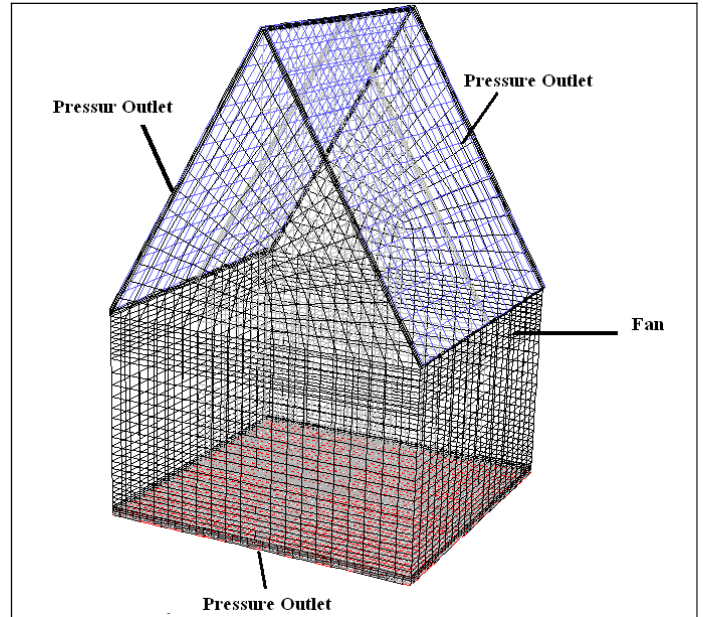
Figure 1- Geometry and the boundary conditions
