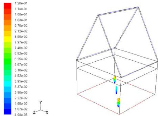
Fig.6 Injecting droplets in range of 1-5 micrometer
