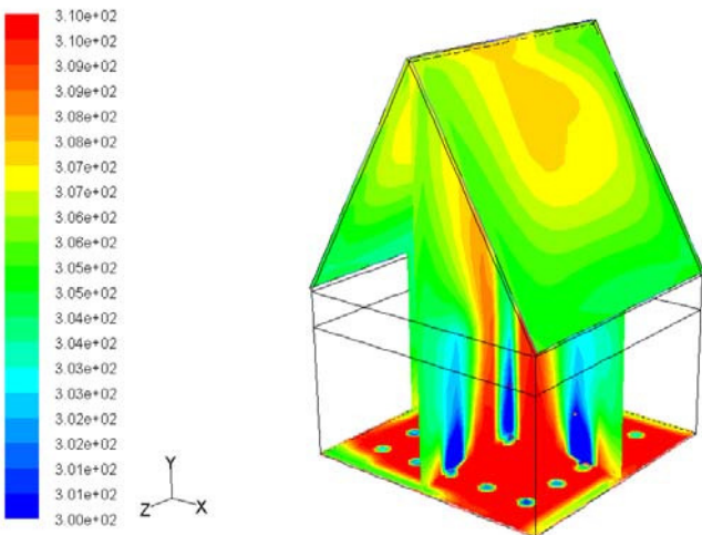
Fig.10 temperature distribution(k) with flow rate 1.8kg/s
