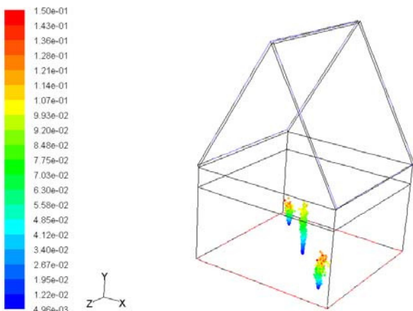
Fig.5 Injecting droplets in range of 1-10 micrometer
