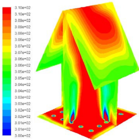
Figure.3 temperature distribution(k) Injecting from 17 points of surface with flow rate 1.27 kg/s
