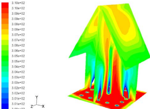
Fig.9 temperature distribution(k) with flow rate 1.7 kg/s
