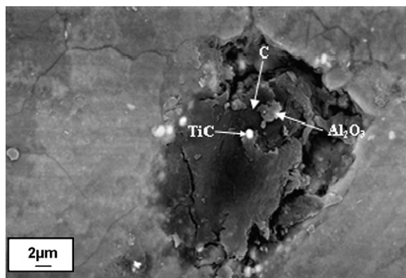
Fig. 4. TiC particle surrounded by retained carbon.
