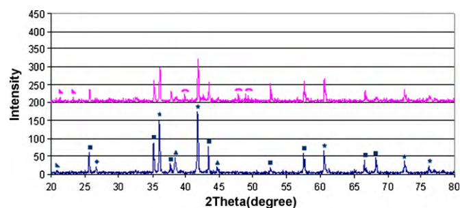
Fig. 1. X-Ray diffractions of sample 6 (upper graph: nano-sample and lower graph: micron sample). (▲) \text{Al}_4\text{O}_4\text{C} , (■) \text{Al}_2\text{O}_3 , (*) TiC, (▲) Al, (◆) C and (●) \text{Ti}_9\text{Al}_{23} .
