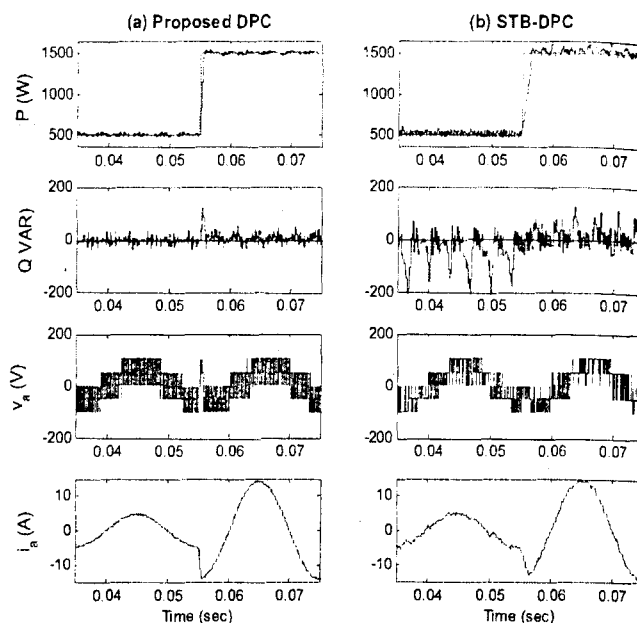
Fig. 4. Simulated waveforms for step change of active power.
