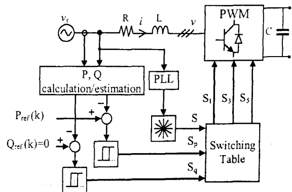
Fig. 1. Block diagram of the conventional DPC.
