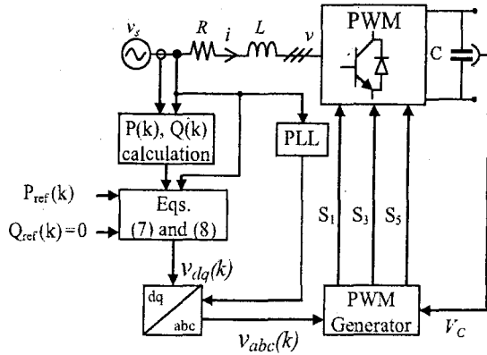
Fig. 2. Block diagram of the proposed DPC.
