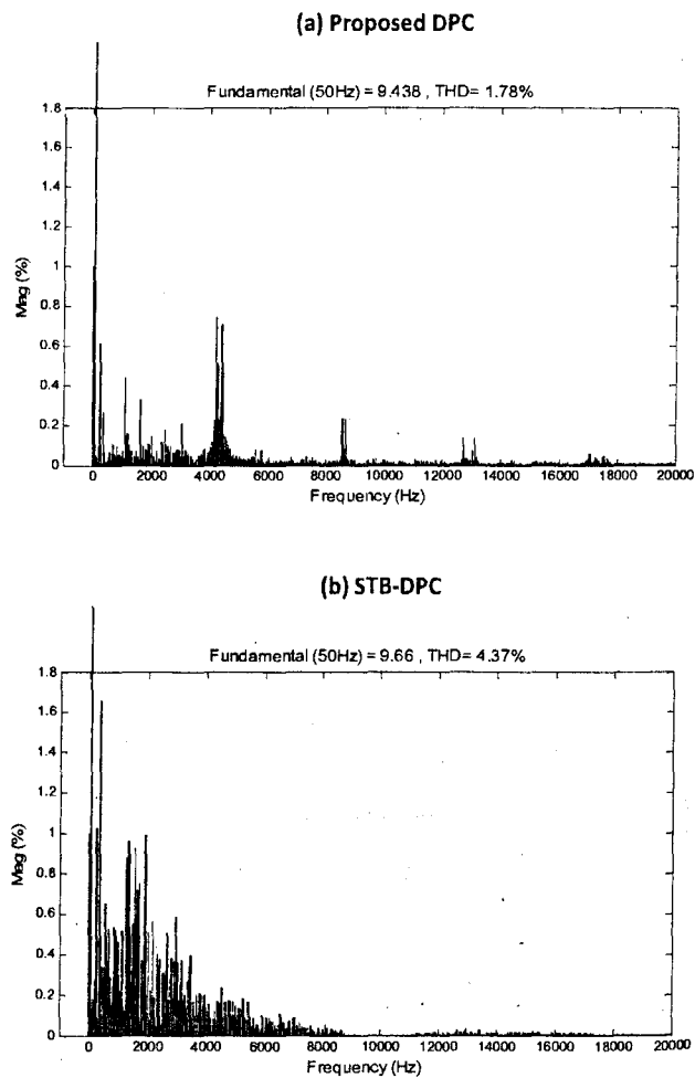
Fig. 5. Simulated line current harmonic spectrum ( P_{ref} = 1000 W, Q_{ref} = 0 )
