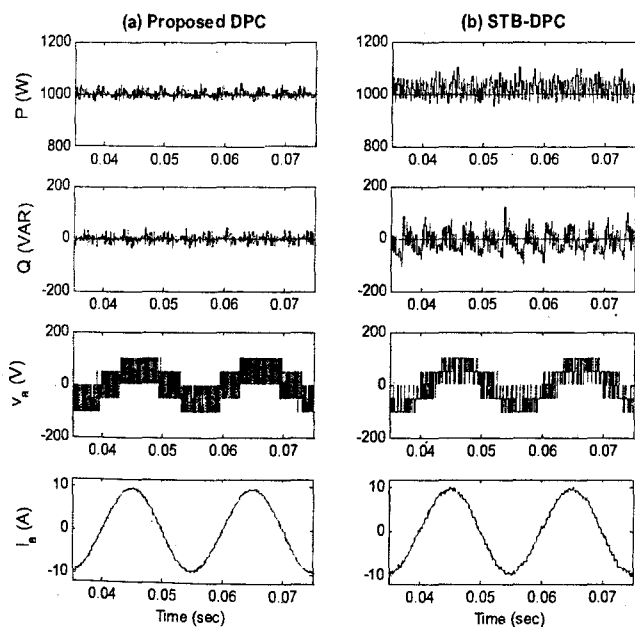
Fig. 3. Simulated waveforms for steady-state operation.
