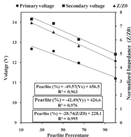
Fig 4. The relations between pearlite percentage and eddy current outputs at 650 Hz.
