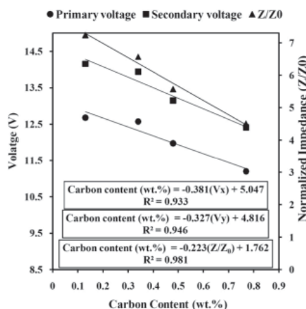
Fig 5. The relation between carbon content of steels and eddy current outputs at 650 Hz.
