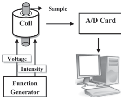
Fig. 1. General synopsis of the experimental apparatus.
