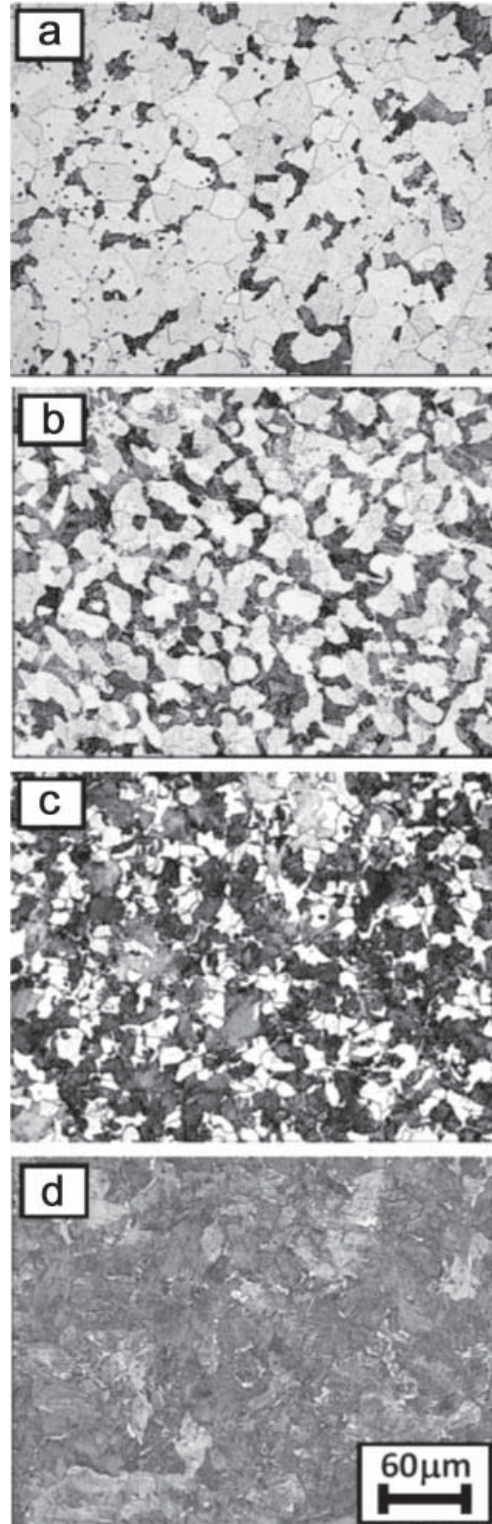
Fig. 2. Metallographic images of AISI a) 1015, b) 1035, c) 1045, d) 1080 steel after full annealing.
