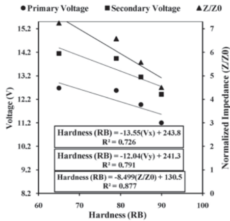
Fig 6. The relation between hardness of steels and eddy current outputs at 650 Hz.
