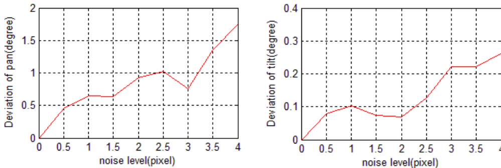
Fig ۷. Standard deviations of the camera rotation at different noise levels
