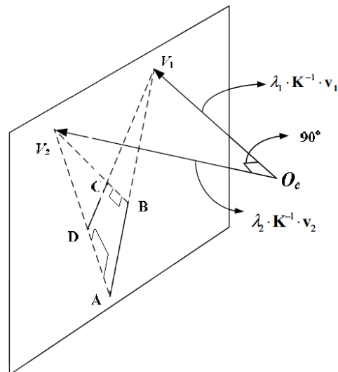
Fig 2. Geometric relationship between vanishing points in the camera coordinates system in sport scene.
