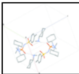
Fig. 2. A view of the hydrogen-bonded centrosymmetric cluster, containing two phosphonic triamide anions and two N -methylcyclohexyl ammonium cations. The N—H...O hydrogen bonds are shown as dotted lines. The H atoms not involved in hydrogen bonding have been omitted for the sake of clarity.
