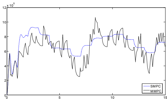
Figure 7. Generator power
