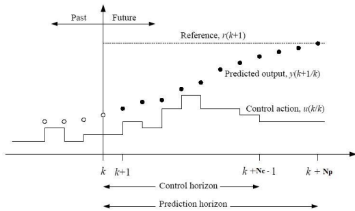
Figure 3. MPC principle
