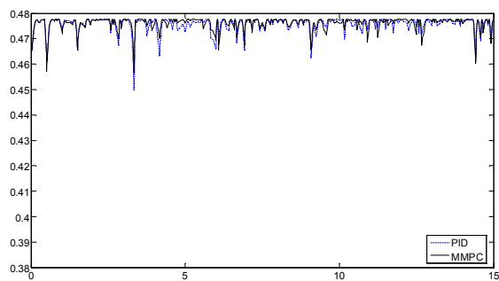
Figure 14. Power coefficient
