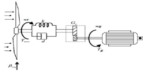
Figure 2. Wind turbine drive train dynamics
