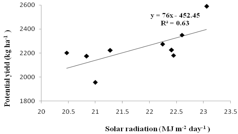
Figure 4. Association of long-term mean simulated potential yield with mean crop season solar radiation among selected regions across Razavi Khorasan.
