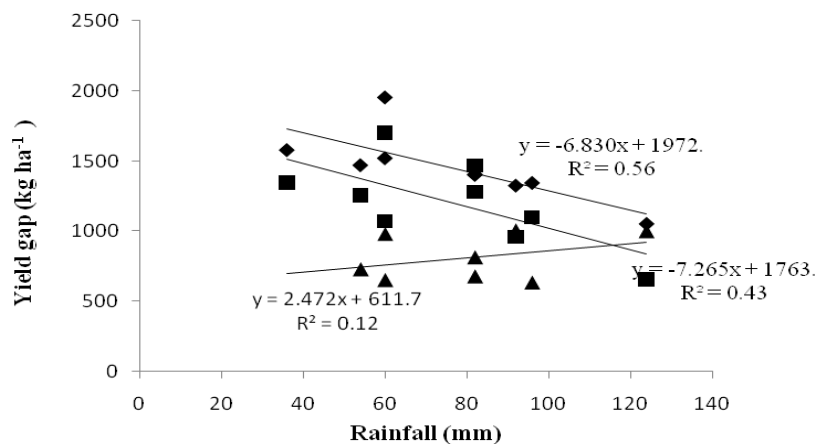
Figure 6. Association of long-term mean yield gap between simulated potential and irrigated actual yield ( \blacklozenge ), mean yield gap between simulated potential and water limited yield ( \blacksquare ) and yield gap between simulated water limited and rainfed actual yield ( \blacktriangle ) with mean crop season rainfall among selected regions across Razavi Khorasan province.
