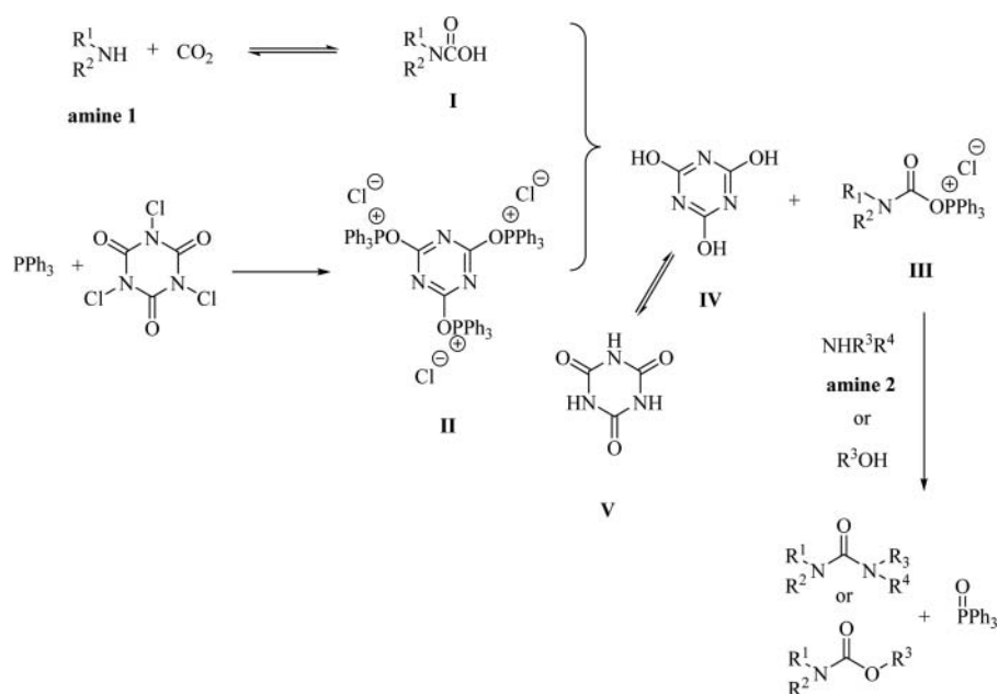
Scheme 2. Proposed mechanism of urea and carbamate synthesis.
