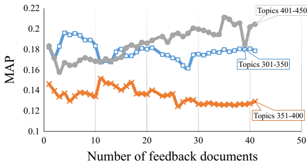
Fig. 4 Tuning the number of extracted articles: MAP over number of extracted articles
