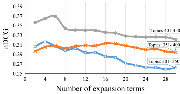
Fig. 3 Tuning the number of expansion terms: nDCG over number of terms
