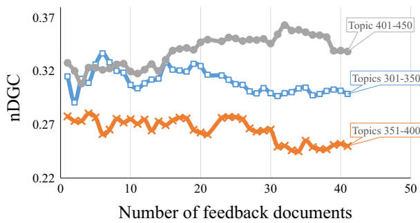
Fig. 5 Tuning the number of extracted articles: nDCG over number of extracted articles
