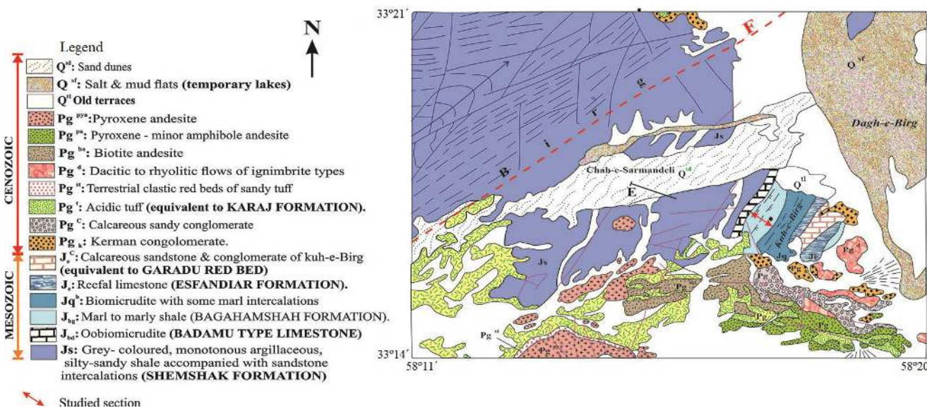
Figure 2. Geological map of the area (part of the geological map 1:100 000 Sarghanj; Lotfi, 1995. Redrawn after Geological Survey of Iran).
